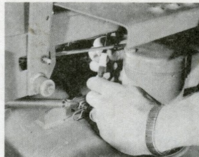
4. Attach mower motor power cables.
