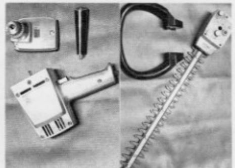
Just like the I-5 Elec-Trak tractor system, the power handle (TM3) accepts a variety of accessories, including the drill head (TH20), and hedge clippers (TH70).
